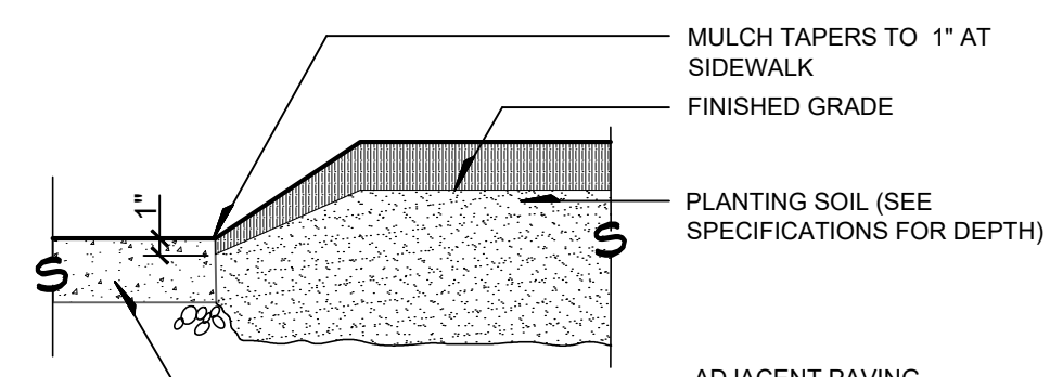
4 PLANT BED EDGE AT PAVEMENT LA.1 SECTION SCALE: 1/2" = 1'-0"
