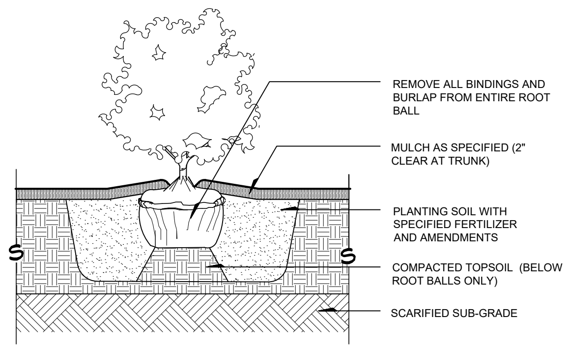
3 TYPICAL SHRUB PLANTING LA.1 SECTION SCALE: 1/2" = 1'-0"
