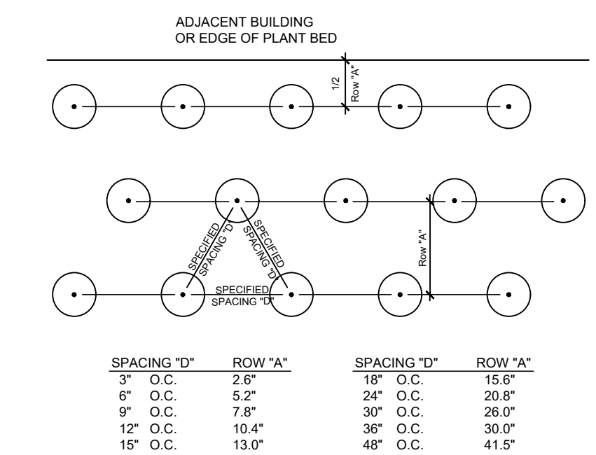
2 GROUNDCOVER SPACING DIAGRAM LA.1 PLAN NTS
